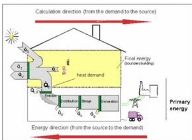
Figure 3: Energy flow and calculation direction
