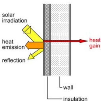
Figure 11: The sketch illustrates the functionality of opaque thermal insulation. Comparison of figures 10 and 11 shows the difference in heat transfer of opaque and transparent insulation.
