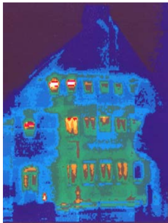
Figure 6: A thermographic picture of a badly insulated façade with thermal bridges.
