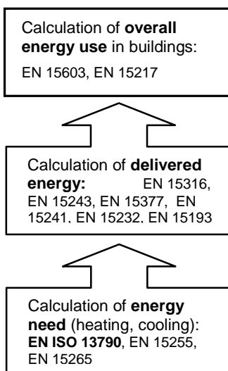
Figure 1: The series of CEN standards offer different types of calculation methods for different steps of the building's energy assessment. EN ISO 13790 includes passive heating and cooling, influencing the energy need.
