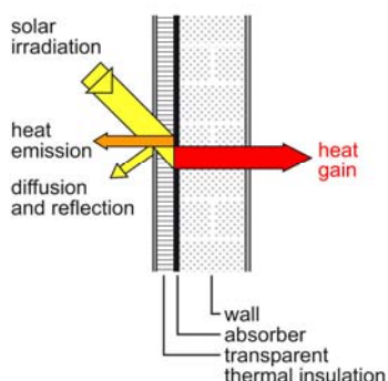
Figure 10: Transparent thermal insulation is not only a good thermal protection, it also allows heat flow of solar energy through the wall (solar heat gains).
