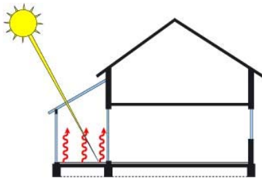
Figure 8: Schematic illustration of direct solar heat gain in an attached but unconditioned sunspace, a conservatory, depicted by the red wavy arrows illustrating heat.
