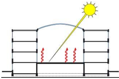
Figure 2: Schematic illustration of direct solar heat gain in an atrium with a glazed roof, depicted by the red wavy arrows illustrating heat.
