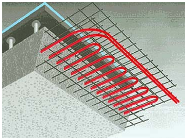
Figure 3: Schematic illustration of a thermo-active ceiling. Cold water can be pumped through the red coloured pipe.
