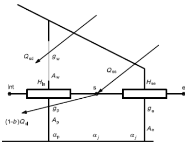
Figure 9: Sketch of an attached sunspace, illustrating direct ( Q_{sd} ) and indirect solar heat gains ( Q_{si} ) and input parameters required for the calculation
